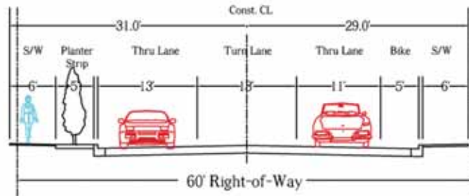
with Planter Strip & Sidewalk
