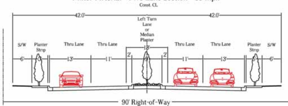
with Planter Strip & Sidewalk
