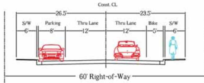
with Parking & Sidewalk
